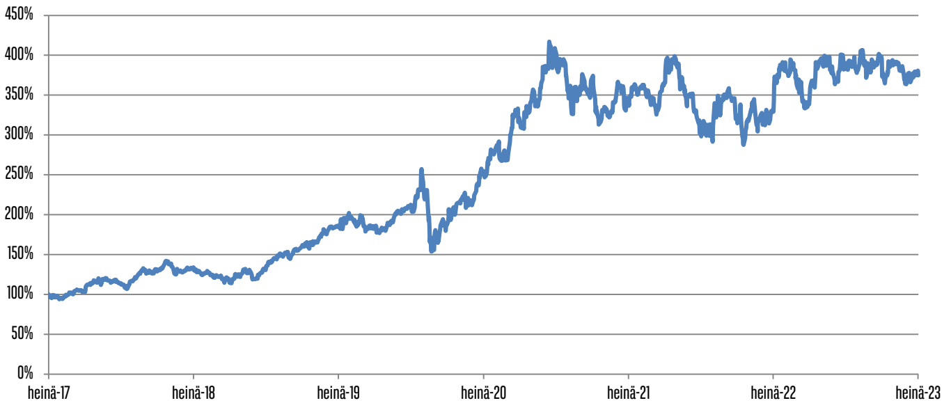
Solactive Energy Transition 2021 Index AR 5%
